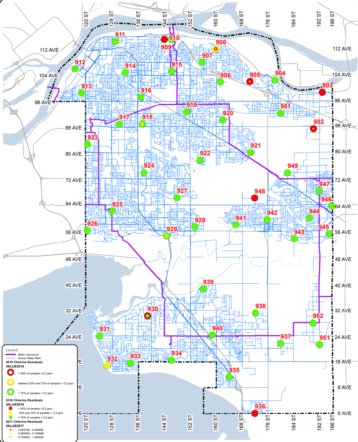
Fig. 6: 2019 CHLORINE RESIDUALS
